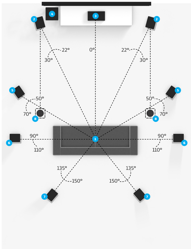
Speaker placement for 9.1.2 setup
