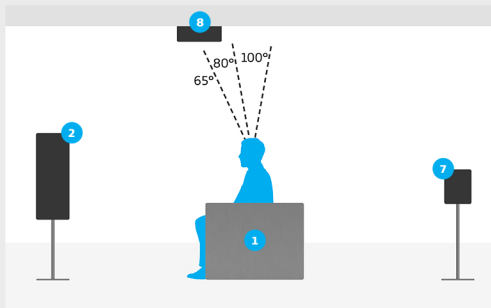
Overhead speaker placement detail for 9.1.2 setup
